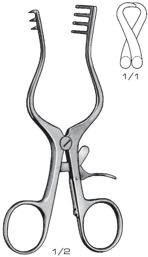
Weitlaner 03-044-13 13 cm / 5 1/8" 03-045-165 16.5 cm / 6 1/2" 3 x 4 Prongs Semi Sharp
