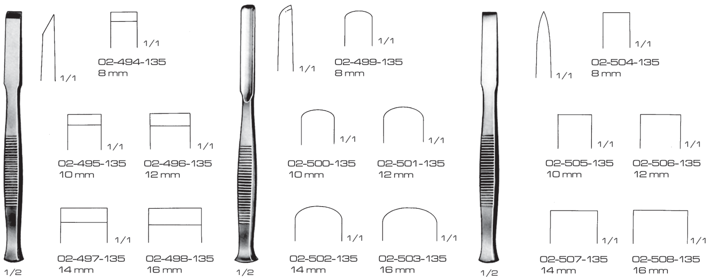
02-494-135 To 02-498-135 13.5 cm / 5¼"
