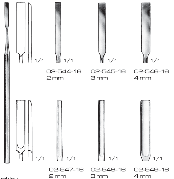
Buckley 02-544-16 To 02-549-16 16 cm / 6 1/4"
