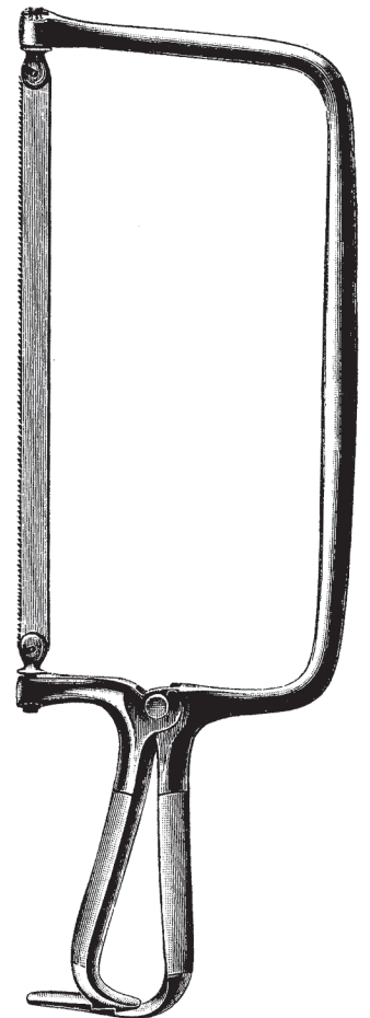
Collin 02-065-33 33 cm / 13 1 / 4 " With 3 blades Blades width 6, 8, 12 mm 02-066-35 35 cm / 14" With 4 blades Blades width 4, 5, 8, 12 mm
