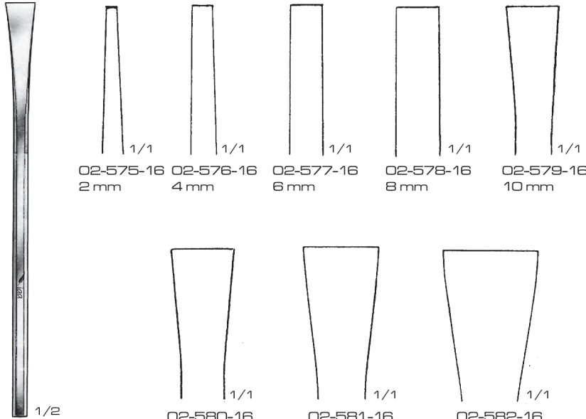
Sheehan 02-575-16 To 02-582-16 16 cm / 6 1/4"
