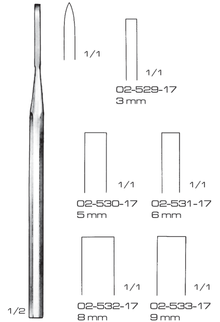
Hoke 02-529-17 To 02-533-17 17 cm / 6 3/4"
