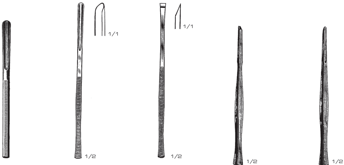
Bishop 02-587-15 2 mm 02-588-15 3 mm 02-589-15 4 mm 02-590-15 5 mm 02-591-15 6 mm 15 cm / 6"
